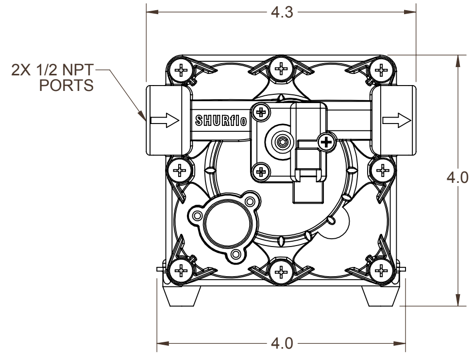
Installation Drawing 94
